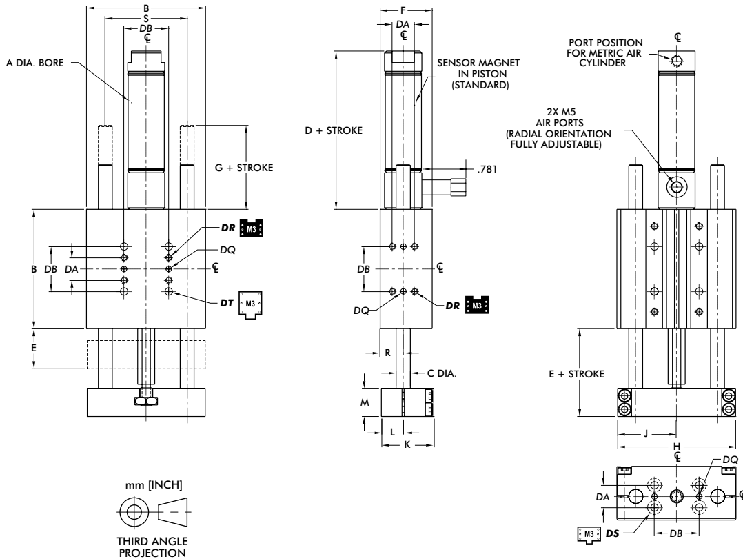
DIRECTCONNECT™ Mounting Pattern Dimensions (all sizes)
